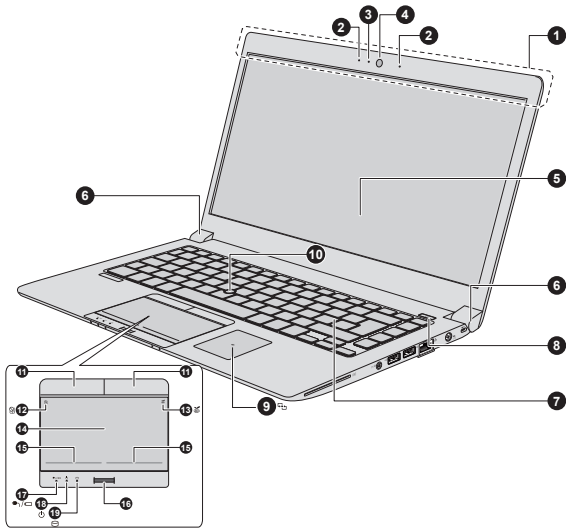
Figure 3-12 The front of the computer with the display panel open (Z40-A)
