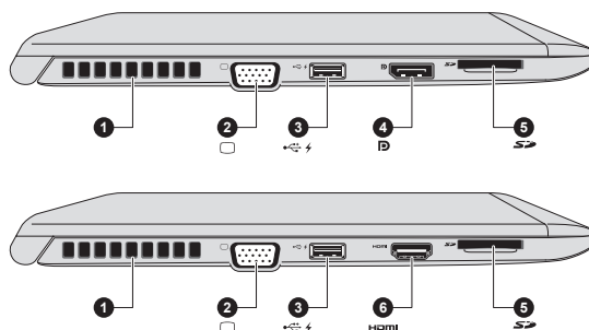
Figure 3-8 The left side of the computer (Z40-A)
